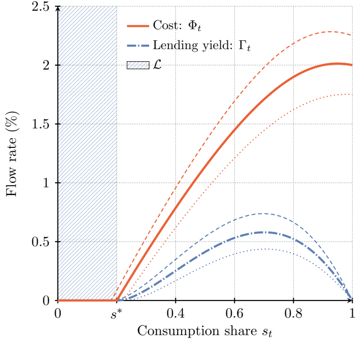
Figure 3: Equilibrium shorting cost and lending yield. The solid and dash-dotted lines represent the equilibrium shorting cost and lending yield as functions of the consumption share of the optimist in a single asset model with \sigma = 0.1 and \delta = 0.05 . The dashed/dotted lines represent the impact of a 10% increase/decrease in the divergence of beliefs \delta .
