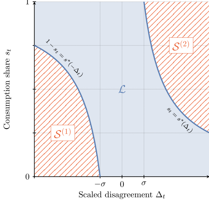
Figure 6: Trading regions with a stochastic disagreement. The figure illustrates the shape of the equilibrium trading regions and allows us to determine the configuration that occurs for each level of disagreement among agents.
