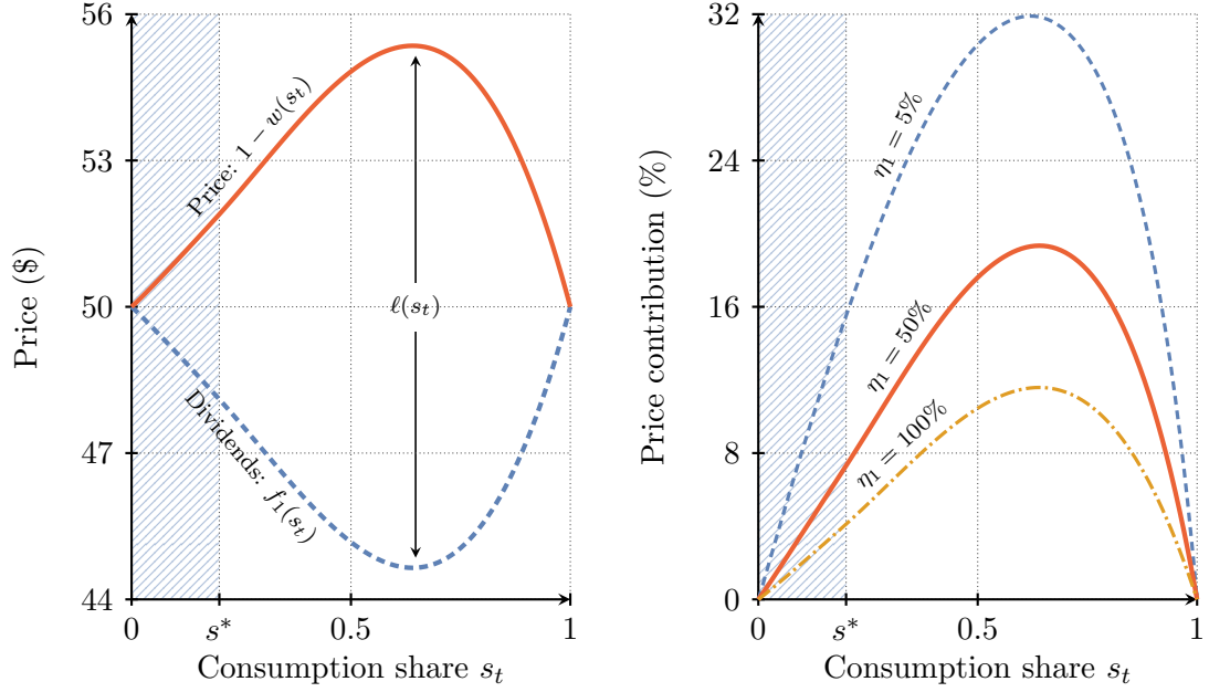
Figure 4: Decomposition of the equilibrium price. The left panel plots the price of the asset 1 (solid line) and the risk-adjusted present value of its dividends (dashed line) when half of the supply is available for shorting. The right panel plots the present value of lending fees as a fraction of the asset price for different values of \eta_1 . In both panels the parameters of the model are set to \sigma = 10\% , \delta = 5\% , \rho = 1\% , e_t = 1 , and the hatched region indicates the interval over which no shorting activity takes place in equilibrium.
