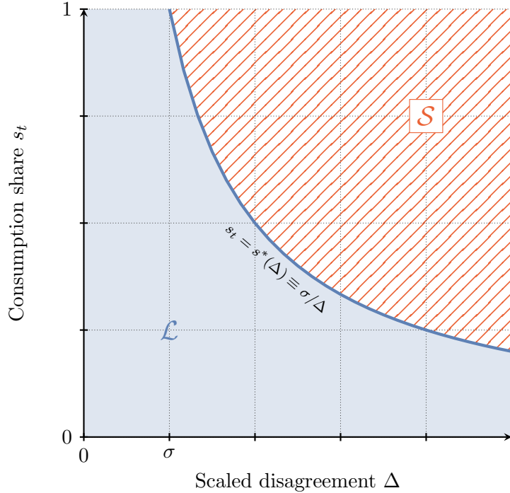
Figure 2: Equilibrium trading regions. The figure illustrates the shape of the equilibrium trading regions and allows us to determine the equilibrium configuration that occurs for each level of disagreement among agents.
