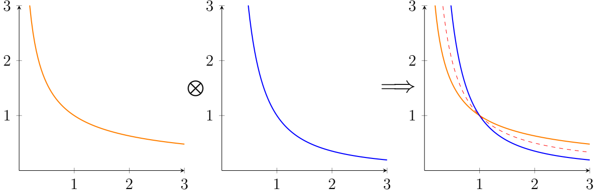
Figure 1: A equally weighted geometric mean of bonding curves where u_1(x, y) = x^{\frac{2}{5}}y^{\frac{3}{5}} , u_2(x, y) = x^{\frac{3}{5}}y^{\frac{2}{5}} and \beta_1 = \beta_2 = \frac{1}{2} .
