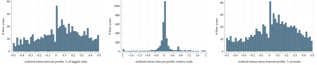
Figure B.1—ALTERNATIVE FORECAST ERROR MEASURES
